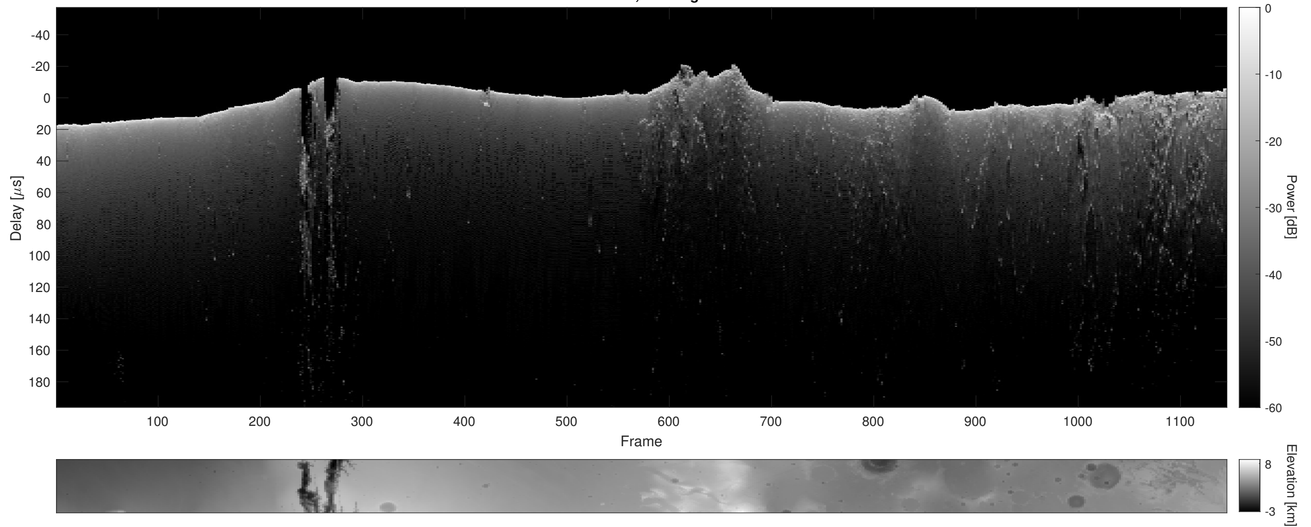
Orbit 15359, Cluttergram
