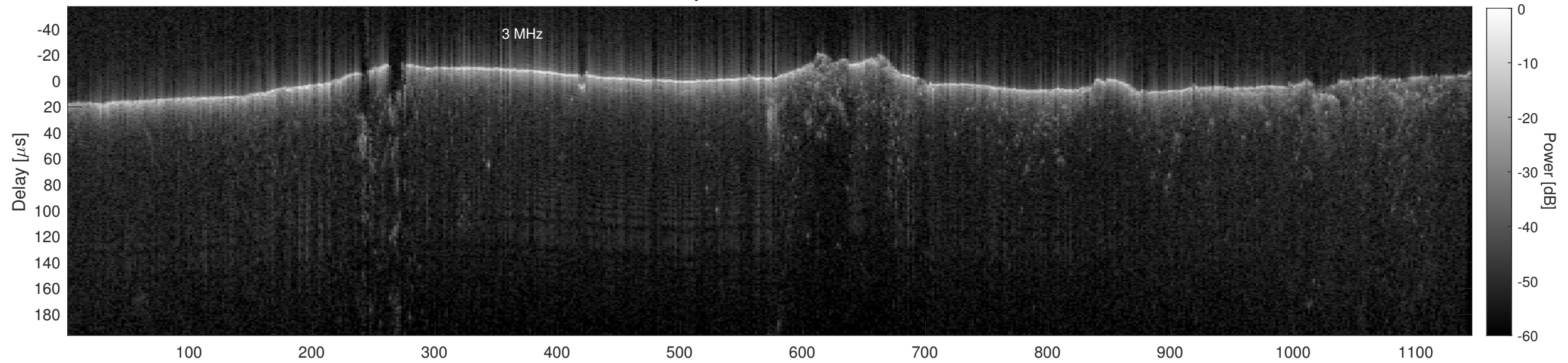
Orbit 15359, Cluttergram
