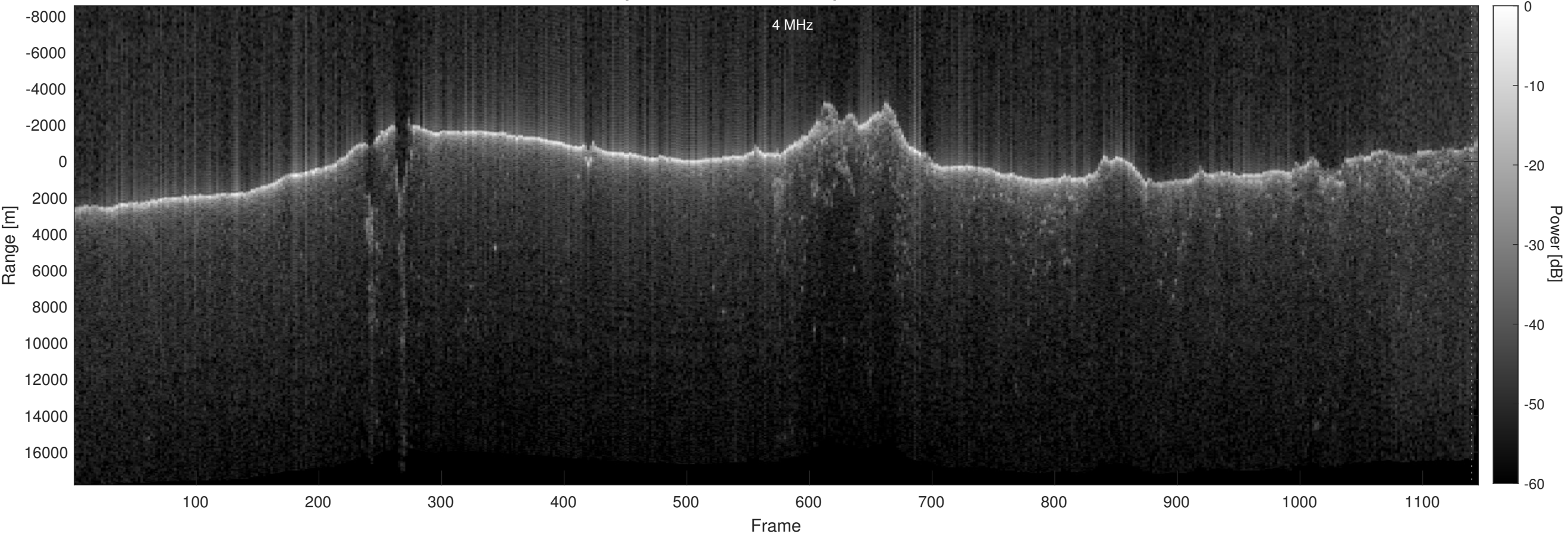
Orbit 15359, Optimized, No Window, Depth-Corrected, Channel 2
