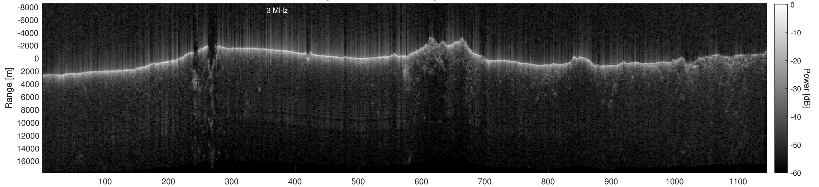
Orbit 15359, Depth-Corrected Cluttergram
