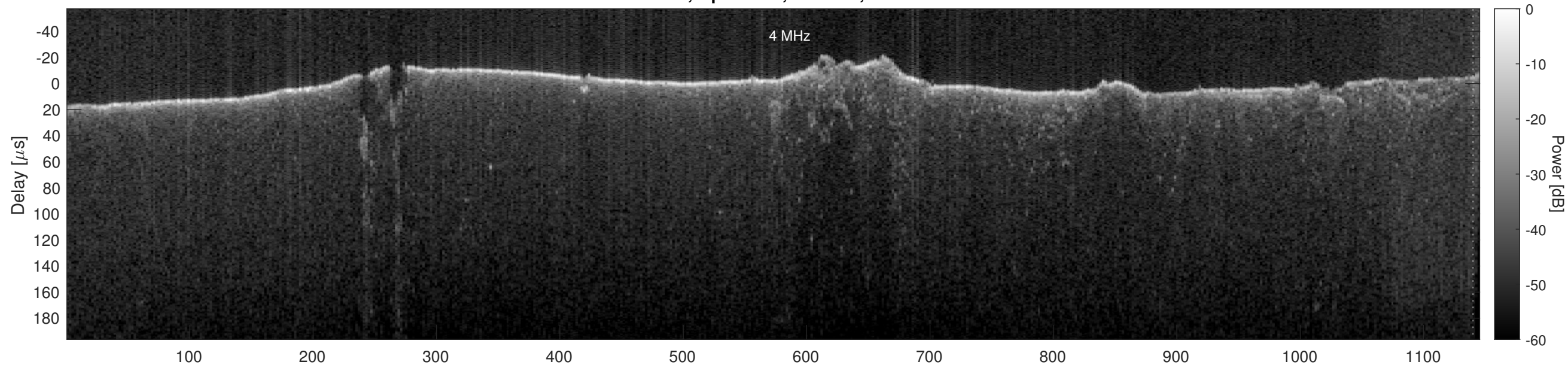
Orbit 15359, Optimized, Window, Channel 2
