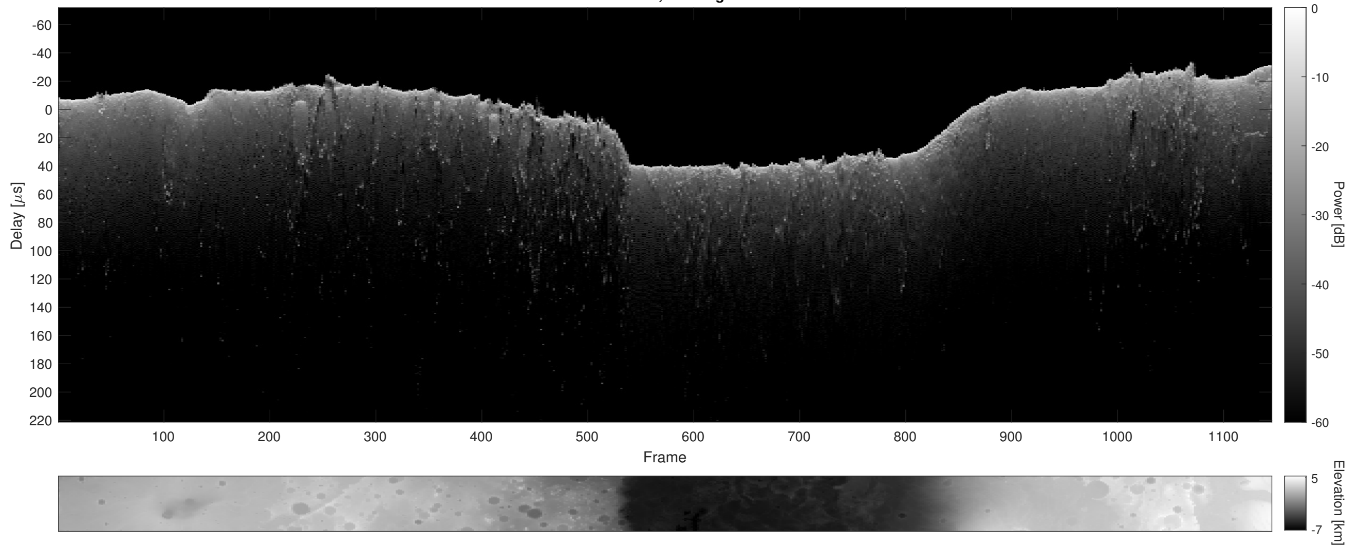
Orbit 15361, Cluttergram
