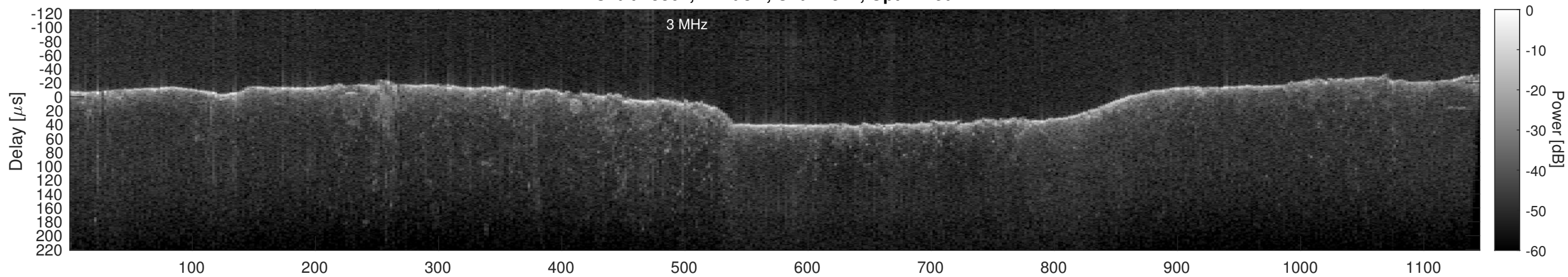
Orbit 15361, Cluttergram
