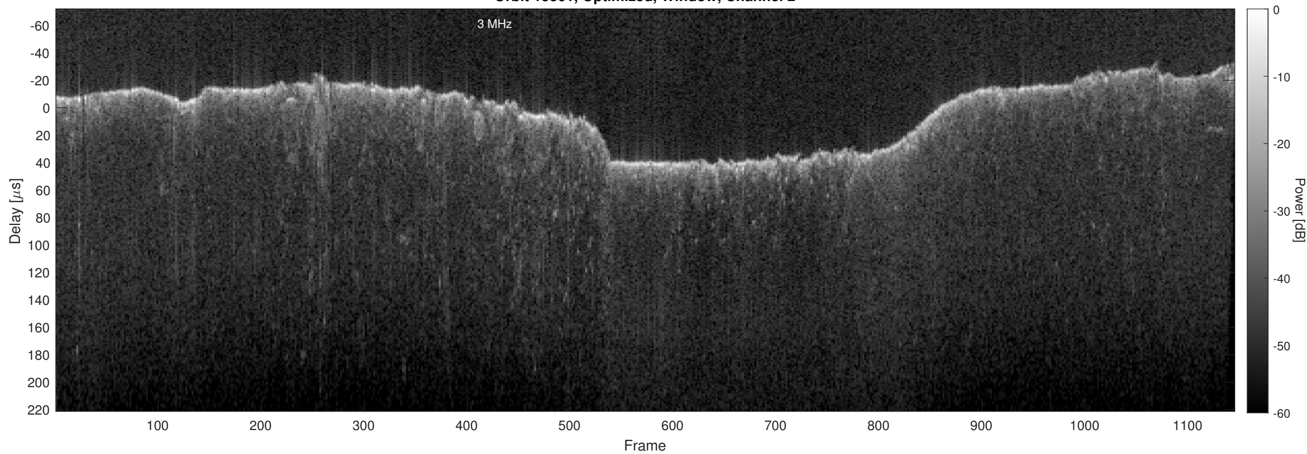
Orbit 15361, Optimized, Window, Channel 2
