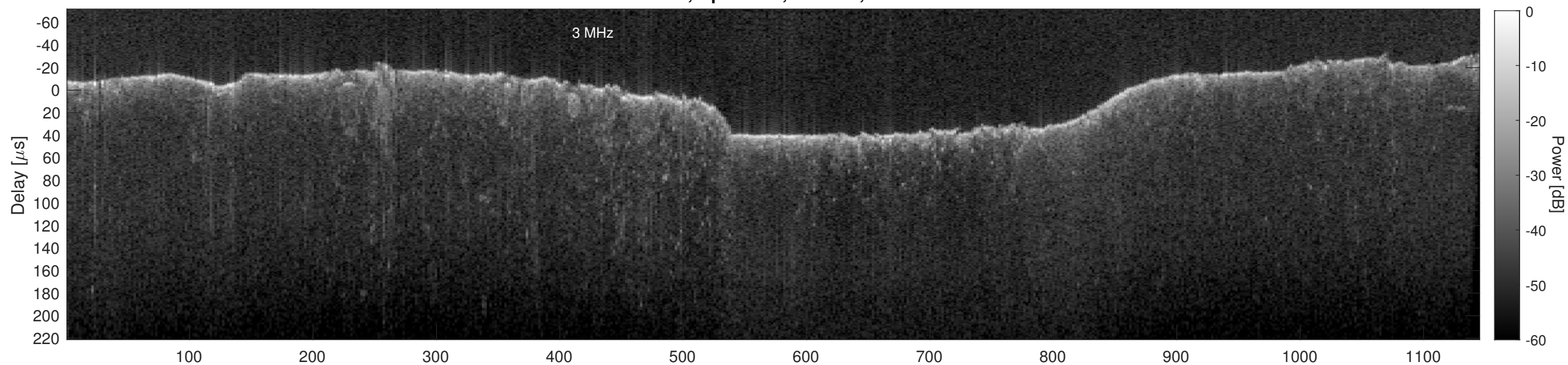
Orbit 15361, Cluttergram
