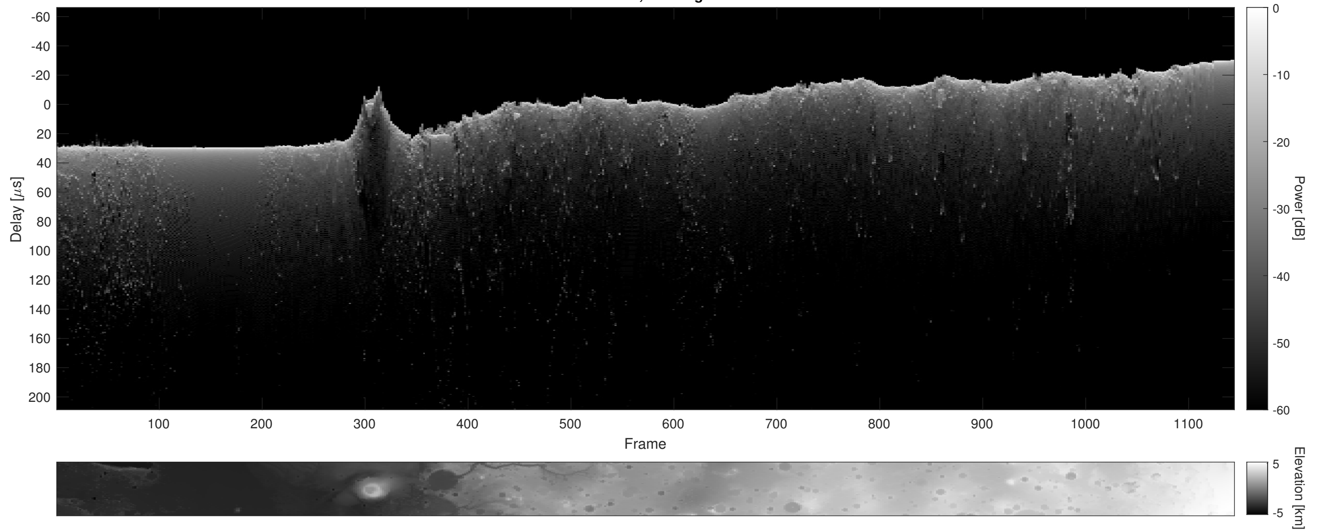
Orbit 15367, Cluttergram
