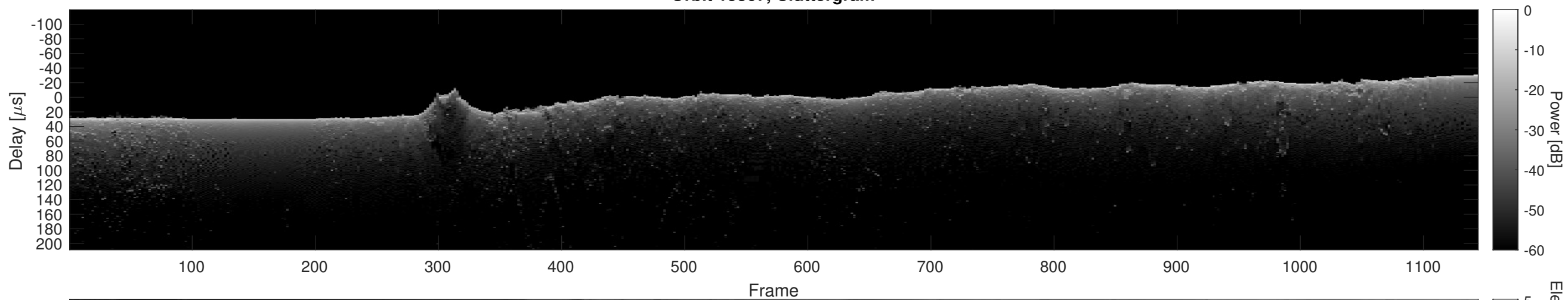
Orbit 15367, Cluttergram
