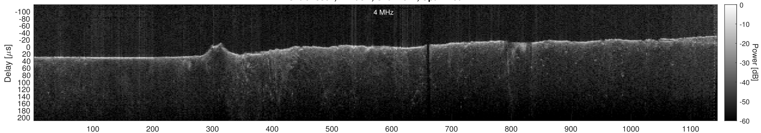
Orbit 15367, Cluttergram
