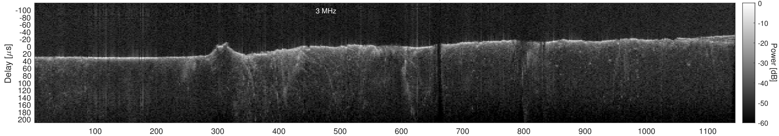
Orbit 15367, Cluttergram
