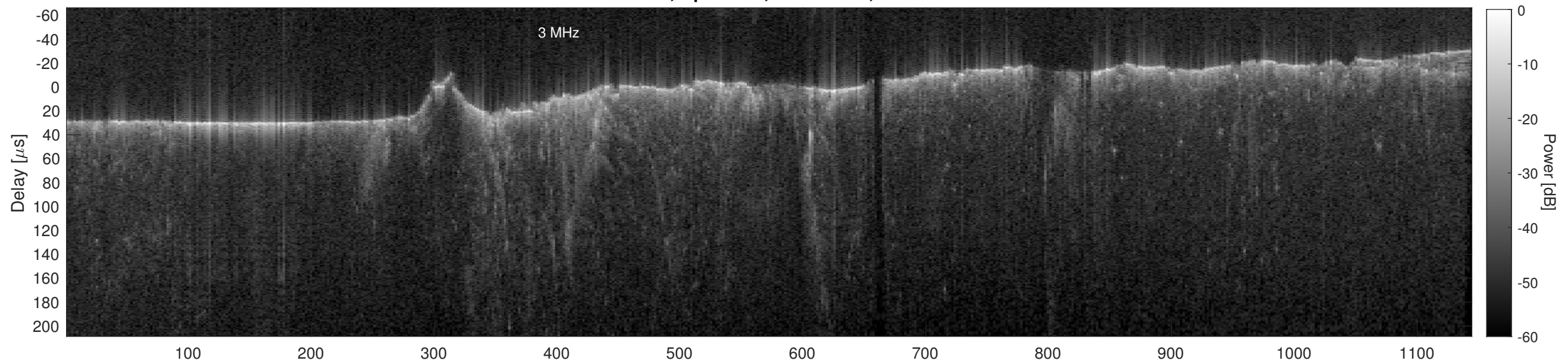
Orbit 15367, Cluttergram
