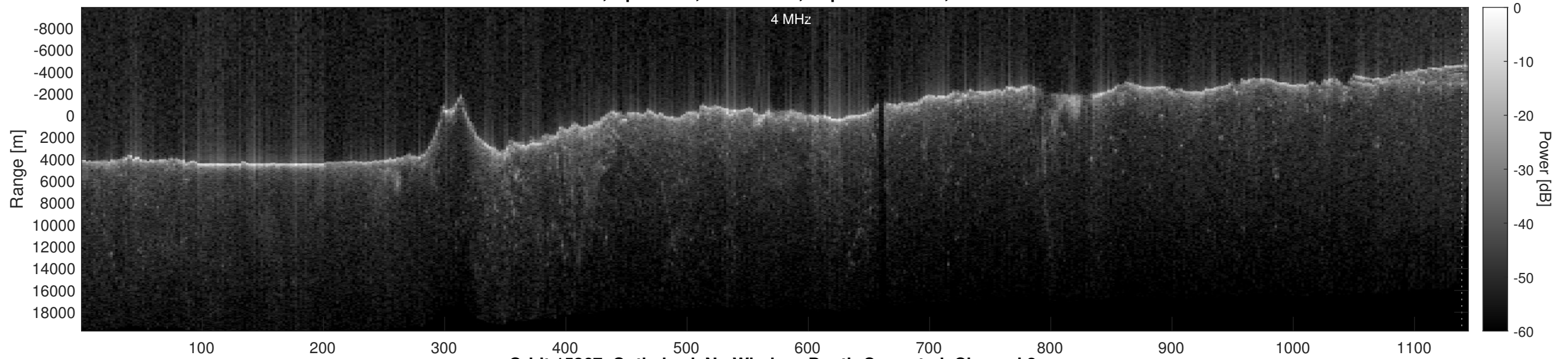
Orbit 15367, Optimized, No Window, Depth-Corrected, Channel 2
