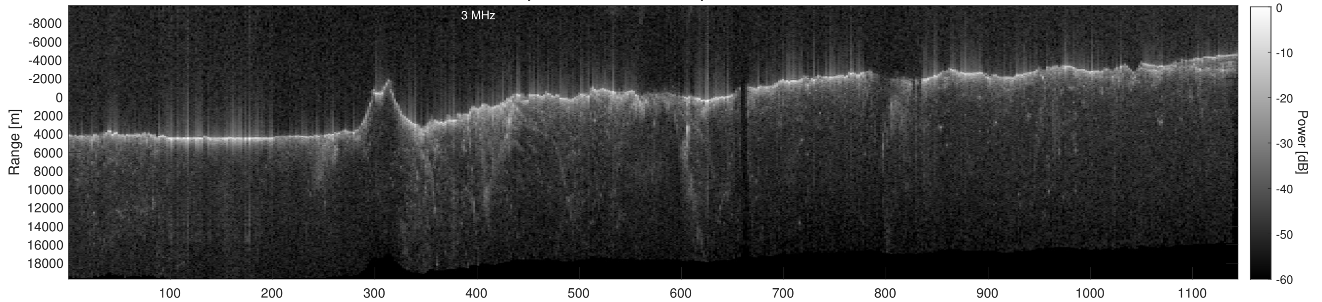
Orbit 15367, Depth-Corrected Cluttergram
