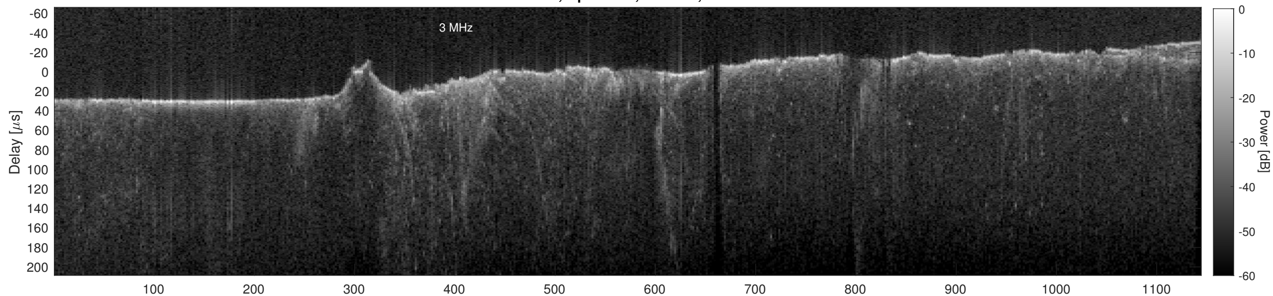
Orbit 15367, Cluttergram
