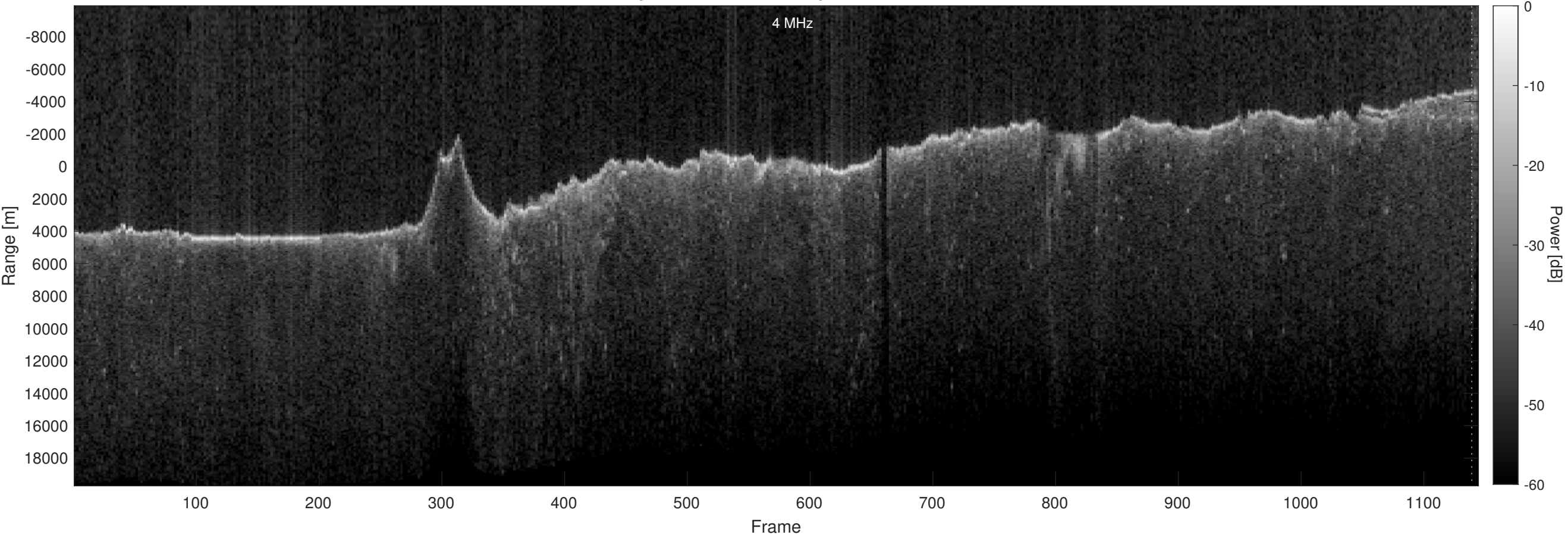
Orbit 15367, Optimized, Window, Depth-Corrected, Channel 2
