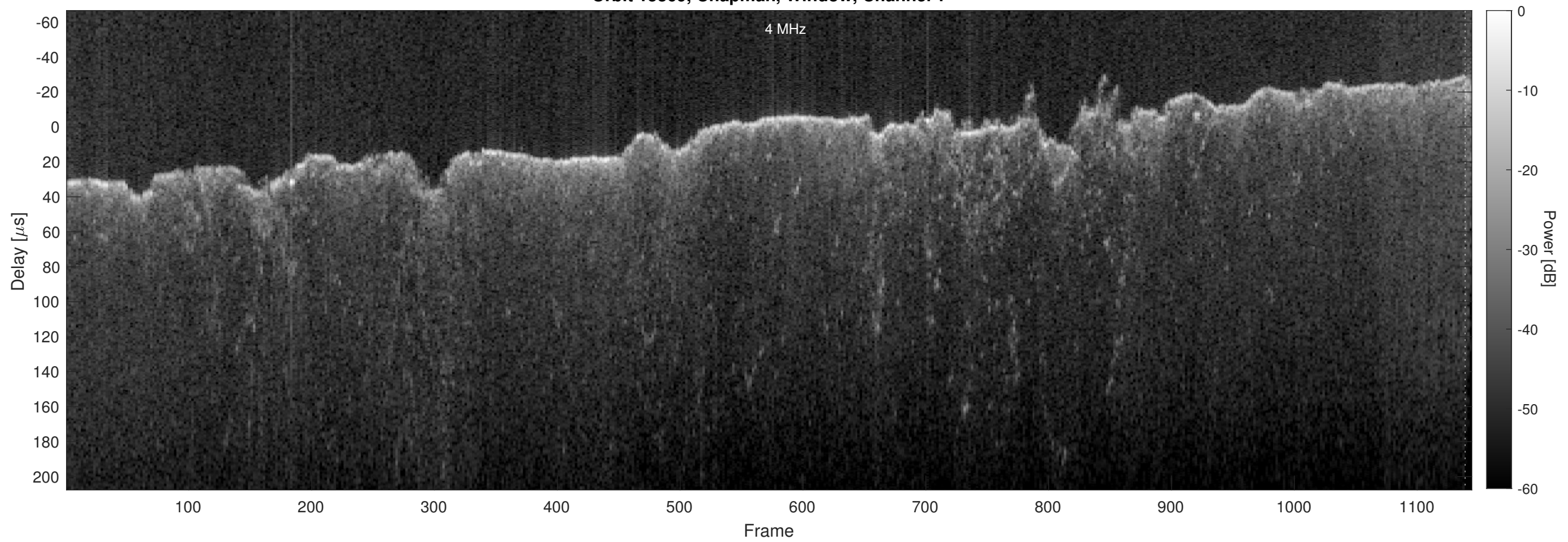
Orbit 15369, Chapman, Window, Channel 2
