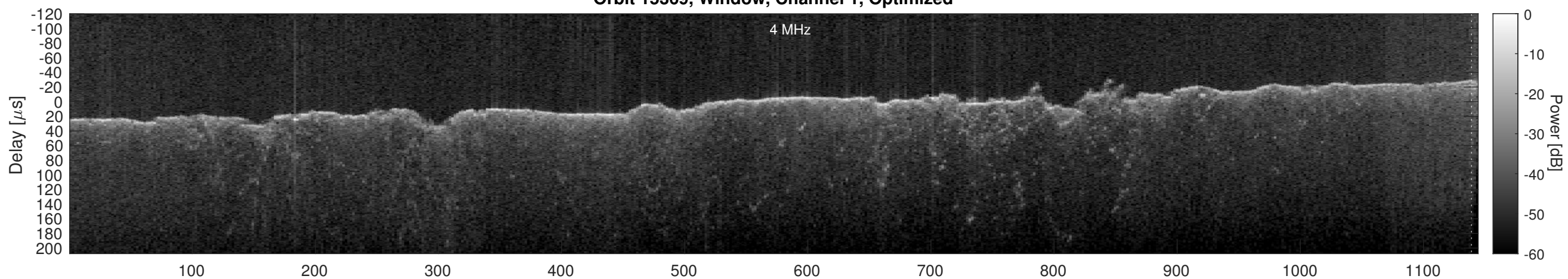
Orbit 15369, Cluttergram
