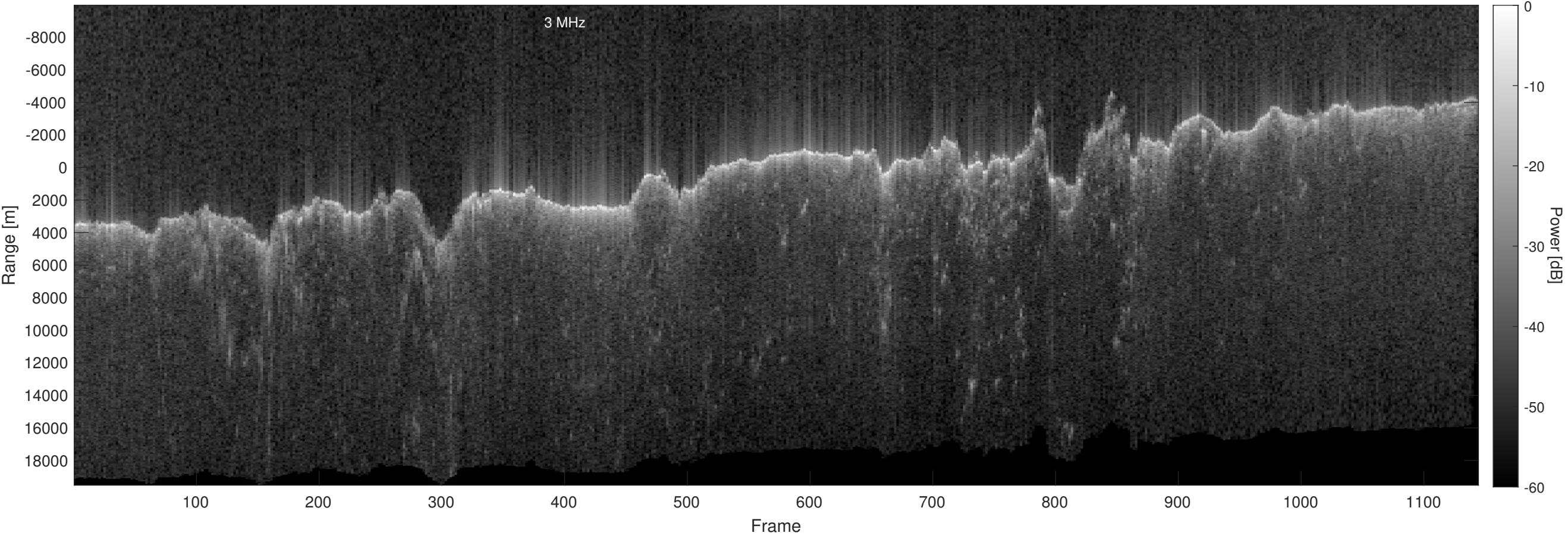
Orbit 15369, Optimized, No Window, Depth-Corrected, Channel 2
