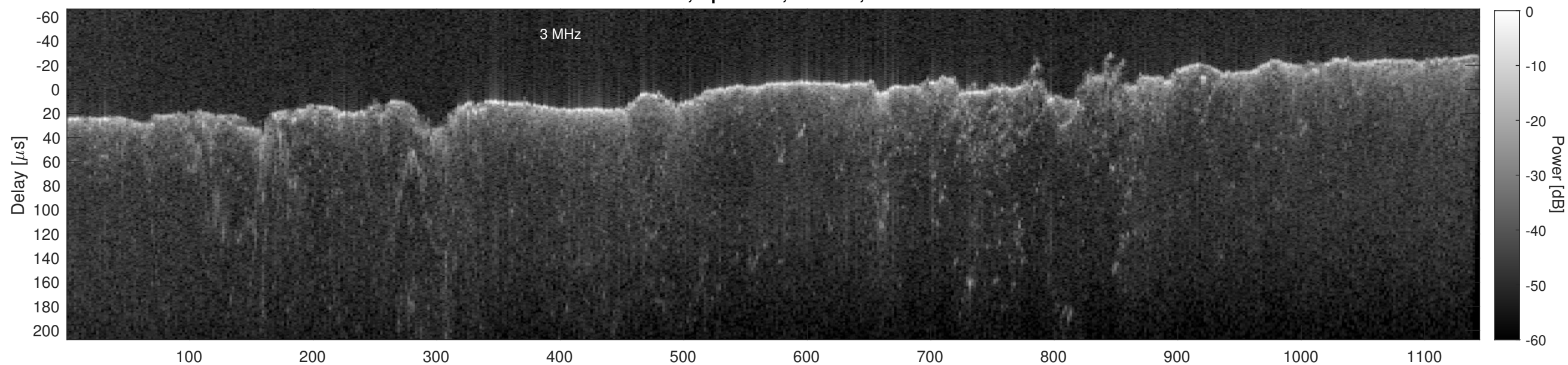
Orbit 15369, Cluttergram
