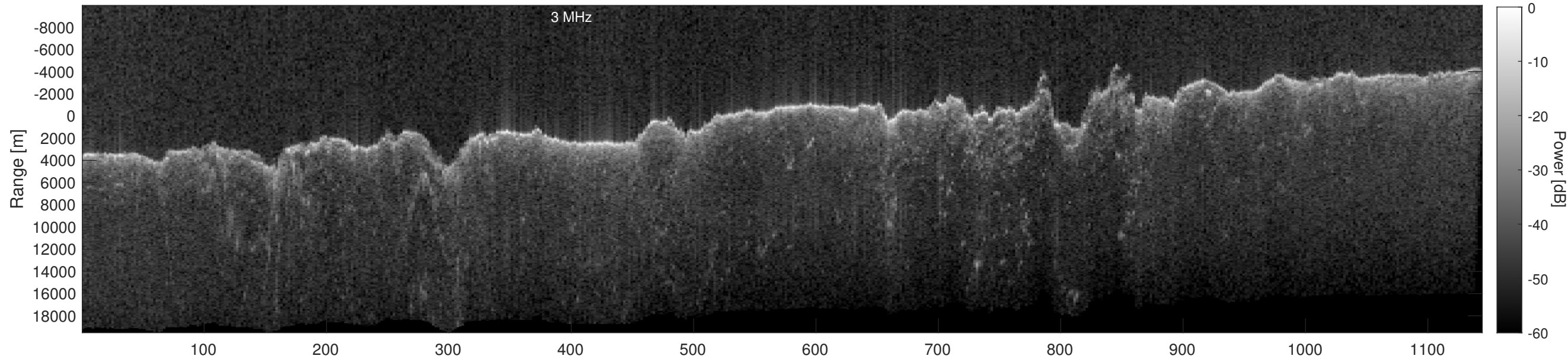
Orbit 15369, Depth-Corrected Cluttergram
