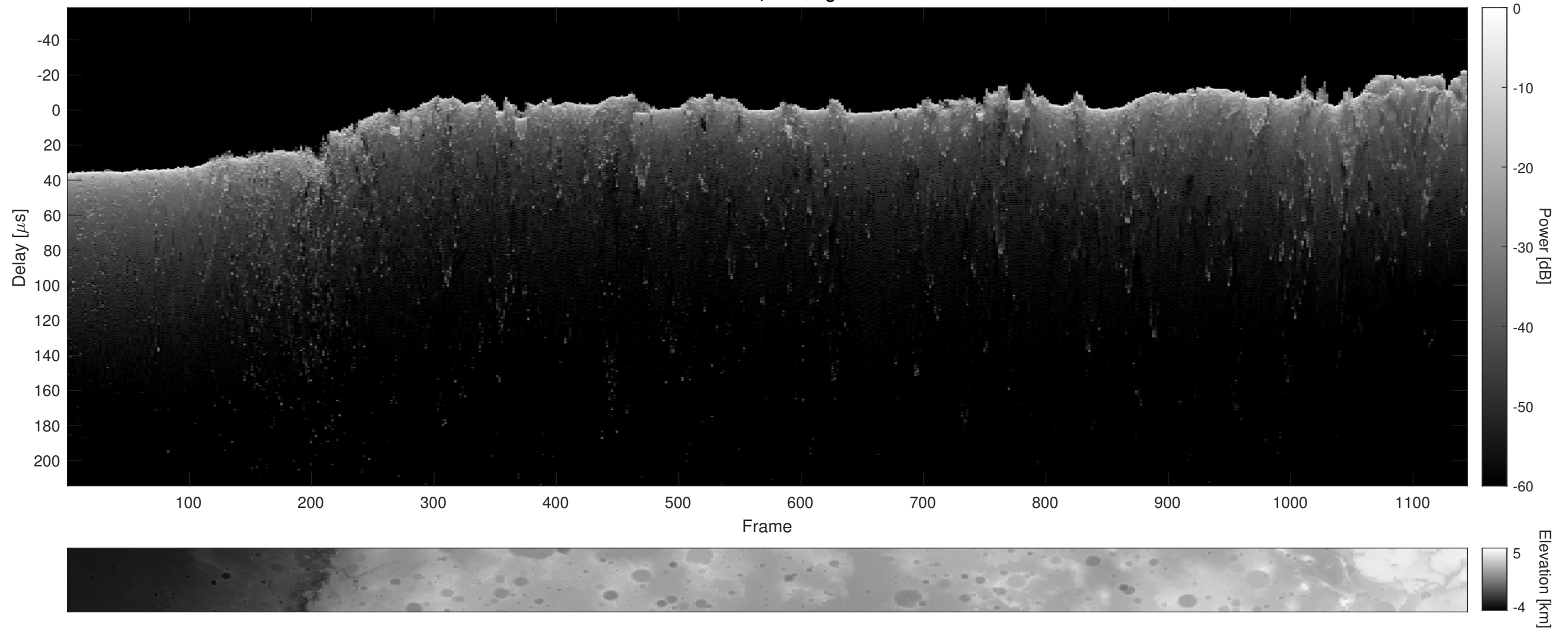
Orbit 15371, Cluttergram
