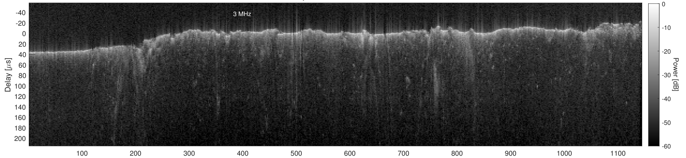
Orbit 15371, Cluttergram
