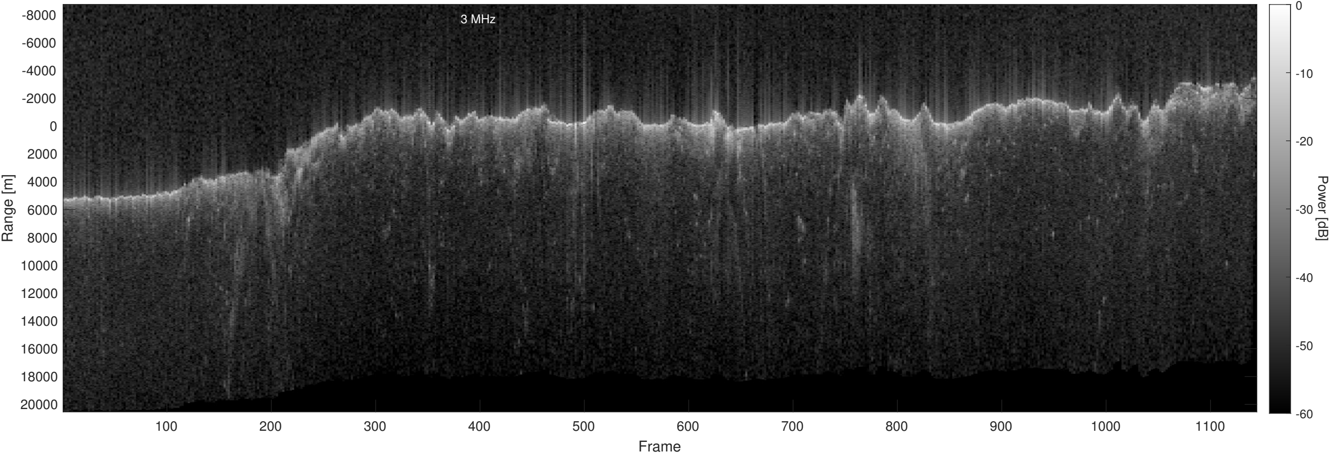
Orbit 15371, Optimized, No Window, Depth-Corrected, Channel 2
