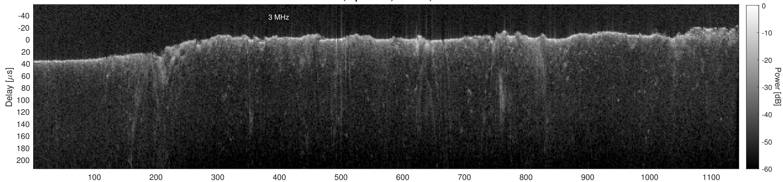
Orbit 15371, Cluttergram
