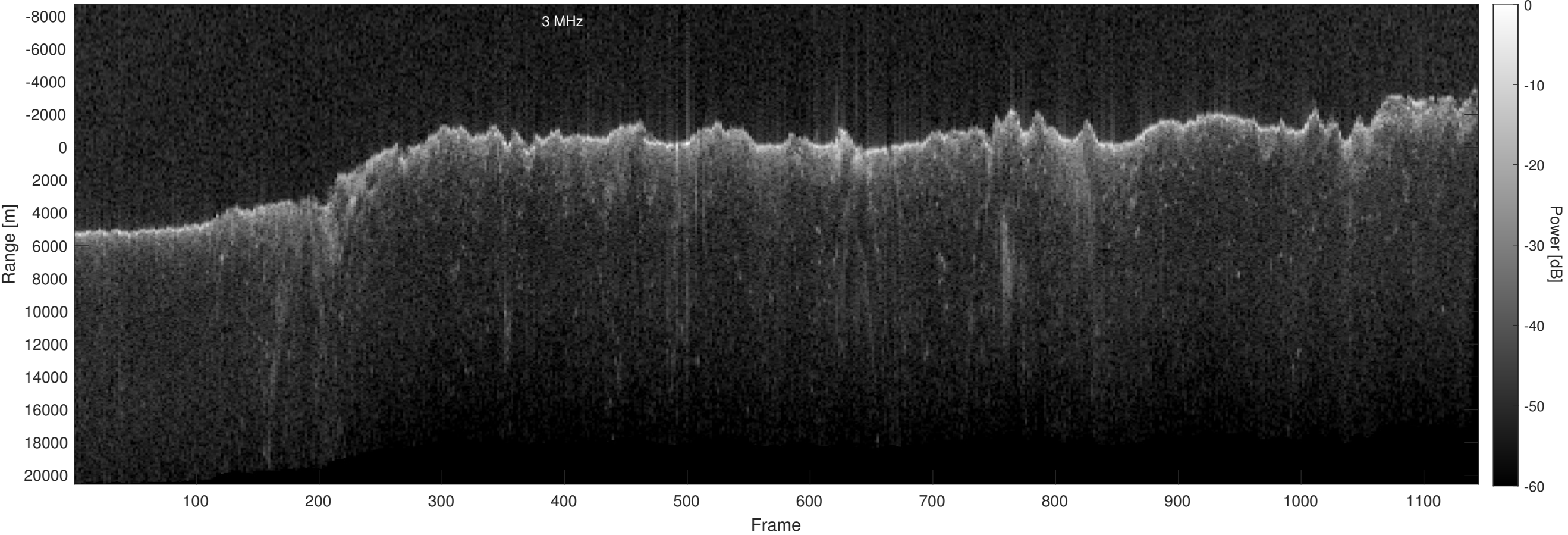
Orbit 15371, Optimized, Window, Depth-Corrected, Channel 2
