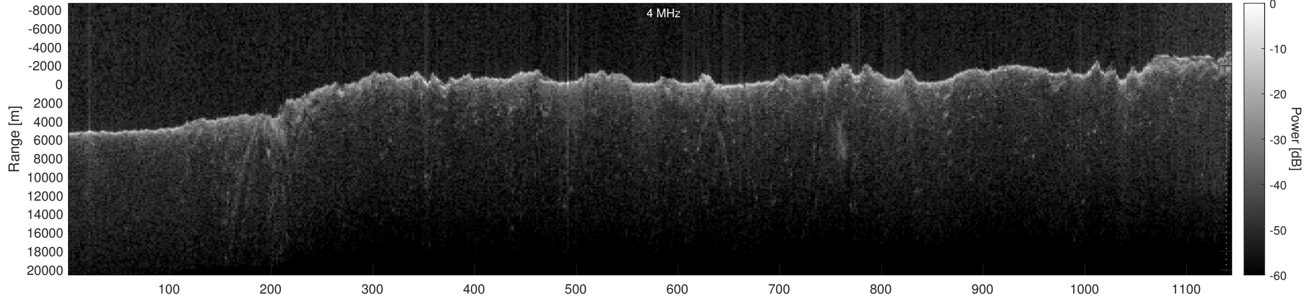
Orbit 15371, Optimized, Window, Depth-Corrected, Channel 2
