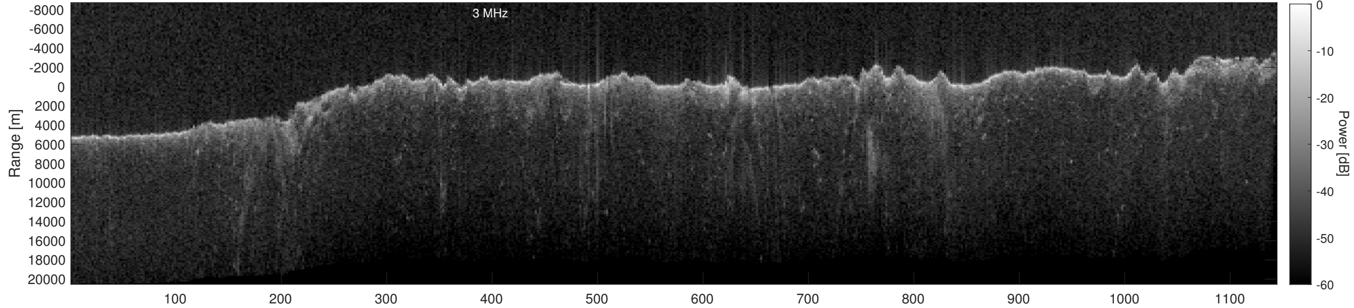
Orbit 15371, Depth-Corrected Cluttergram
