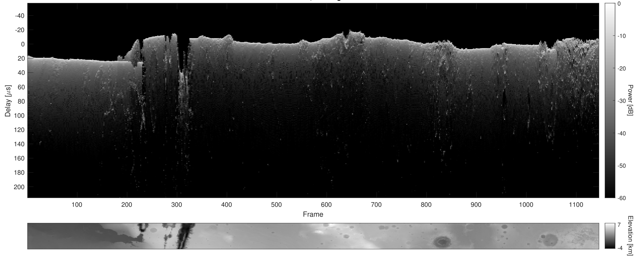
Orbit 15373, Cluttergram
