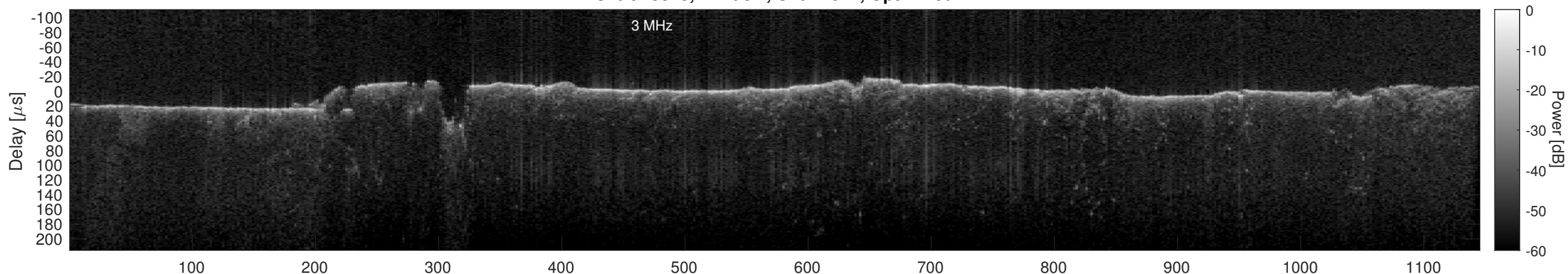
Orbit 15373, Cluttergram
