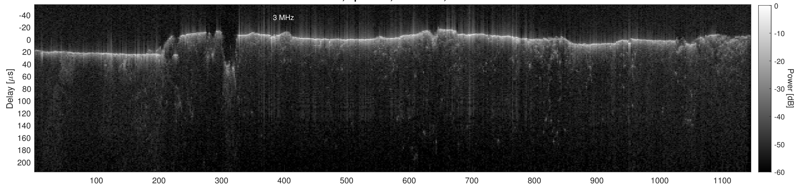
Orbit 15373, Cluttergram
