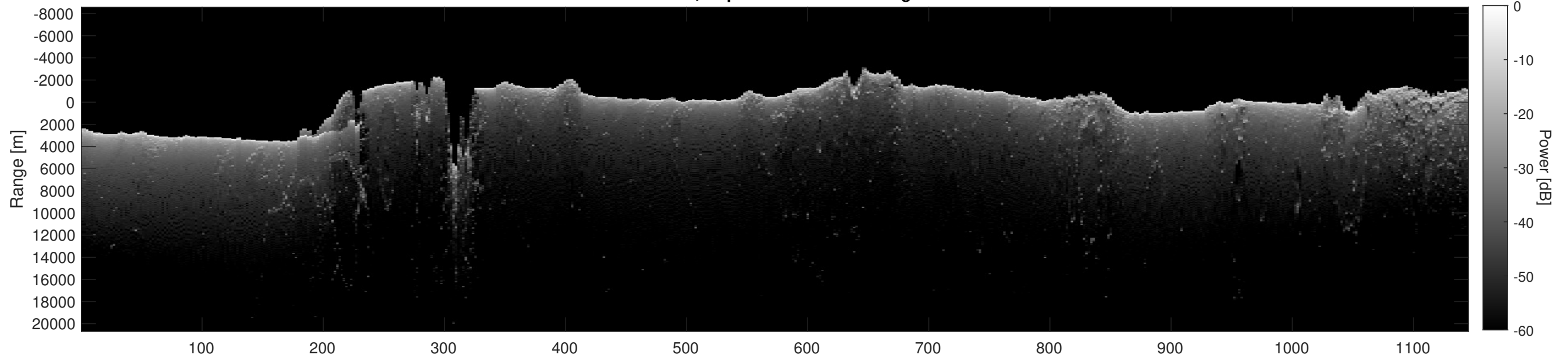
Orbit 15373, Depth-Corrected Cluttergram
