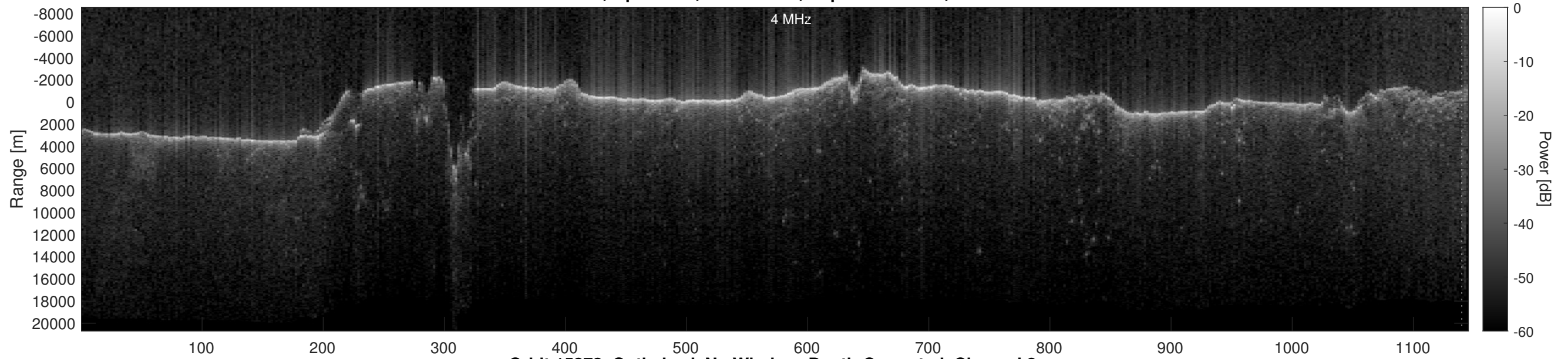
Orbit 15373, Optimized, No Window, Depth-Corrected, Channel 2
