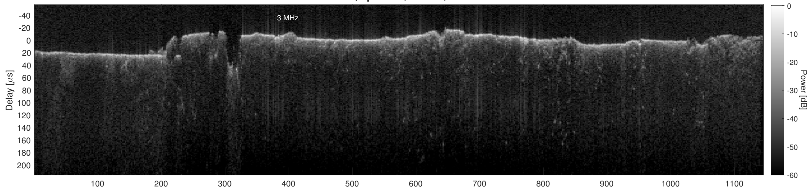
Orbit 15373, Cluttergram
