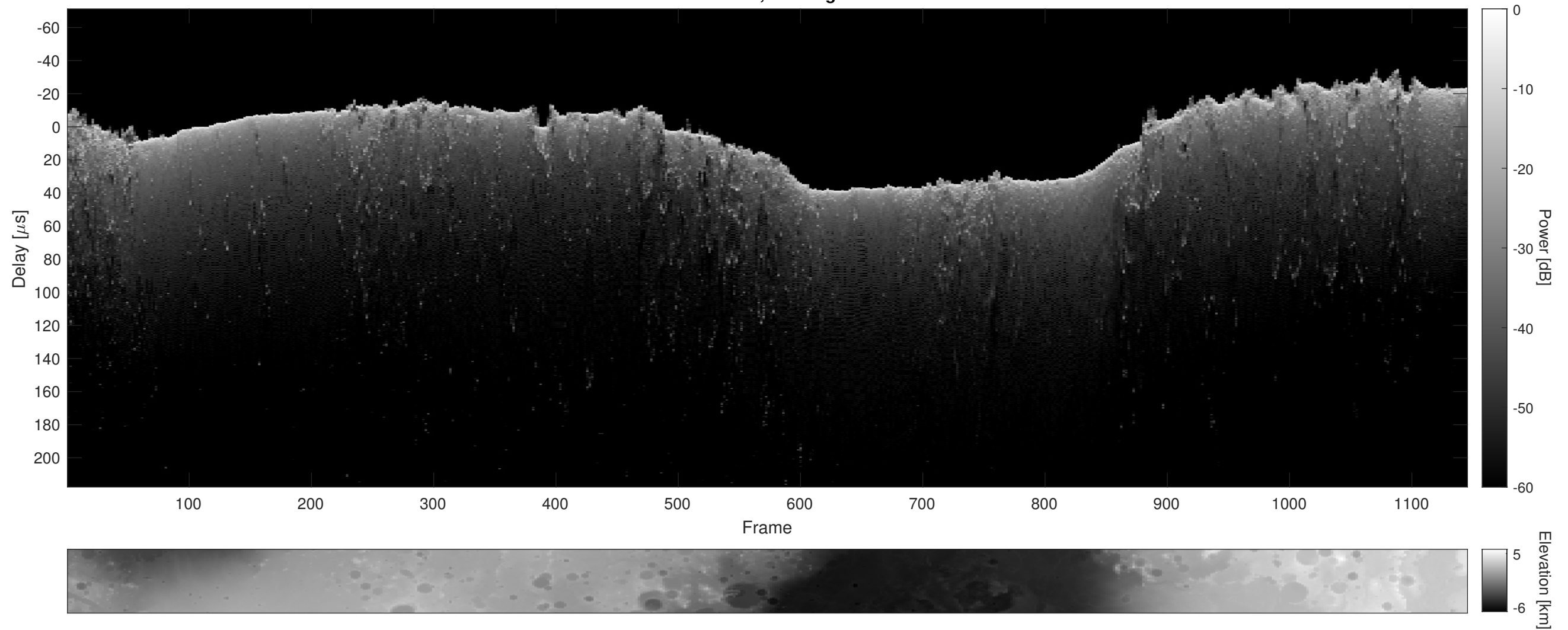
Orbit 15375, Cluttergram
