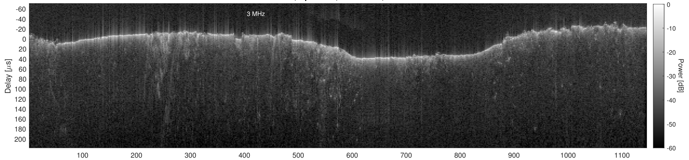
Orbit 15375, Cluttergram
