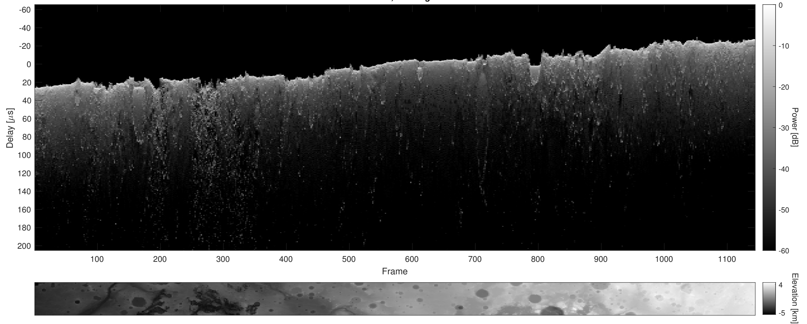
Orbit 15376, Cluttergram
