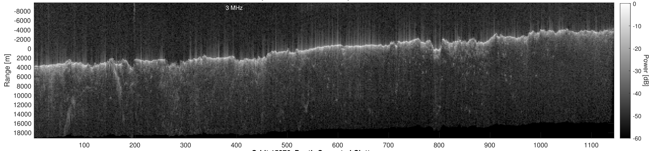
Orbit 15376, Depth-Corrected Cluttergram
