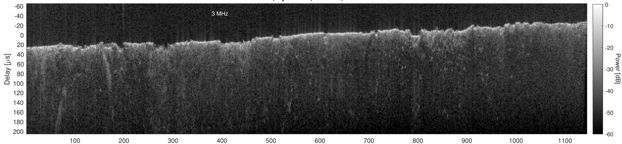
Orbit 15376, Cluttergram
