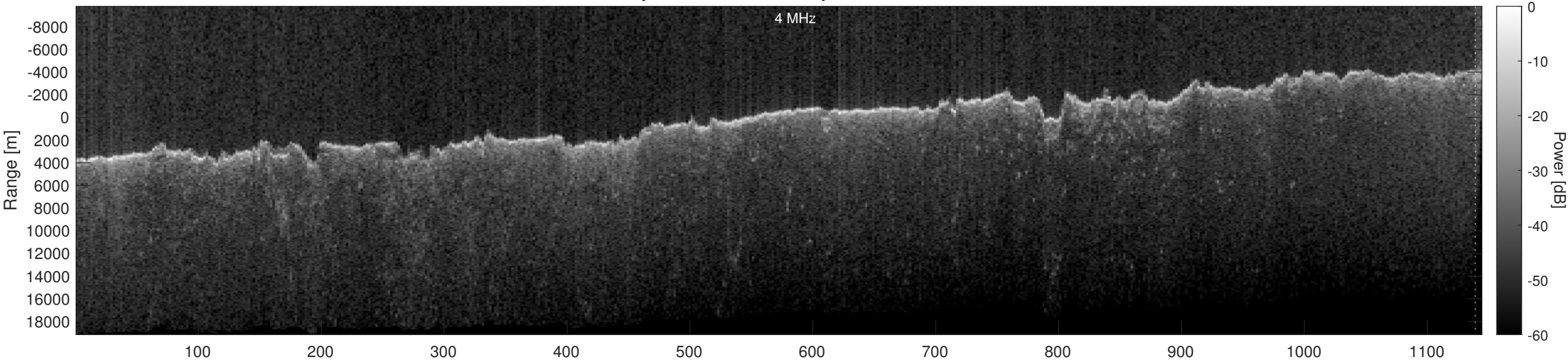
Orbit 15376, Optimized, Window, Depth-Corrected, Channel 2
