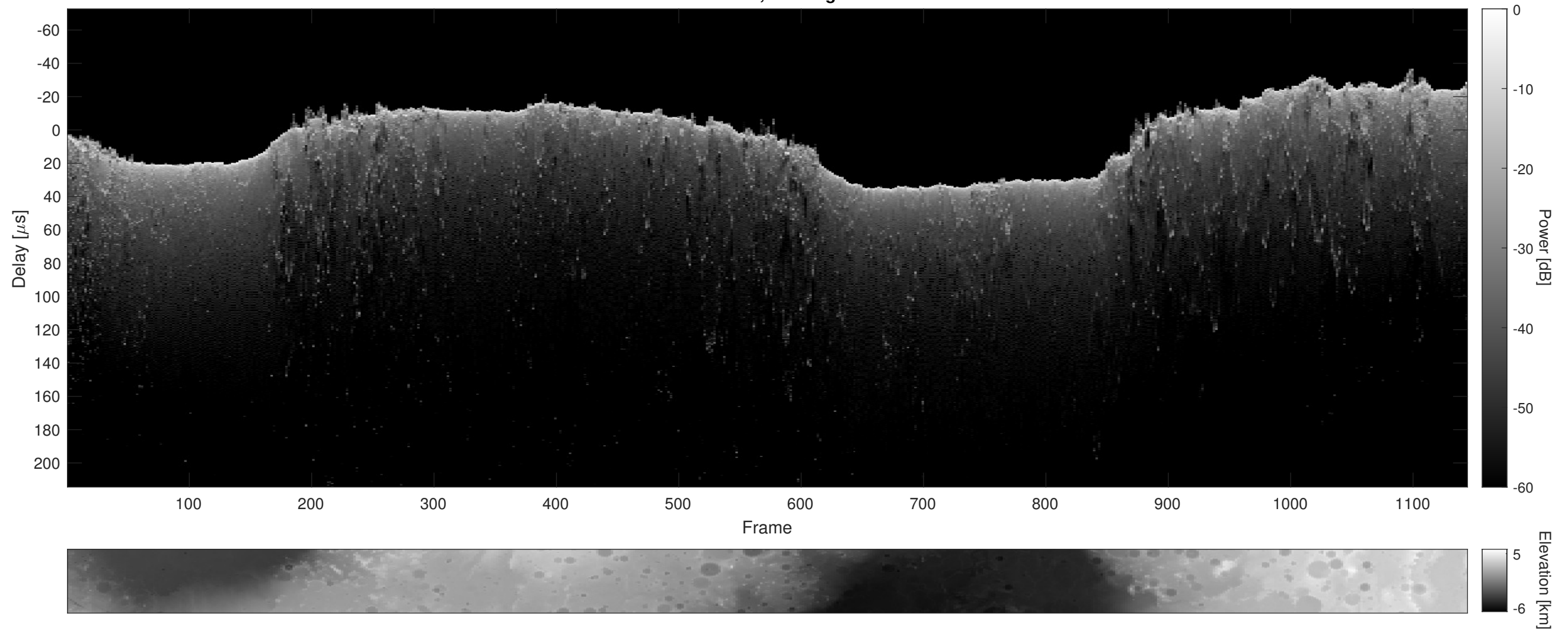
Orbit 15382, Cluttergram
