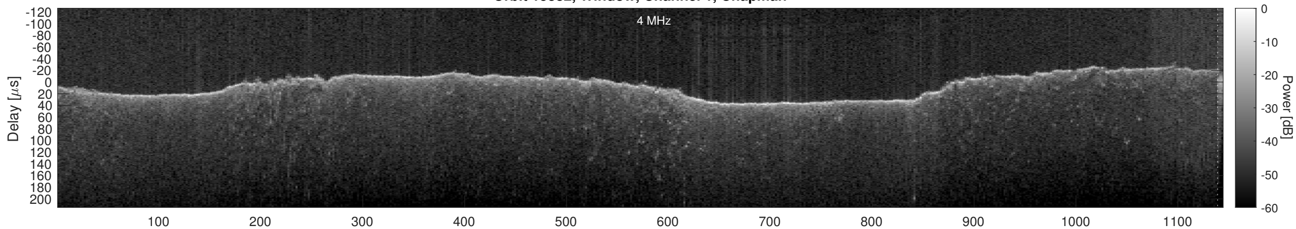
Orbit 15382, Window, Channel 1, Optimized
