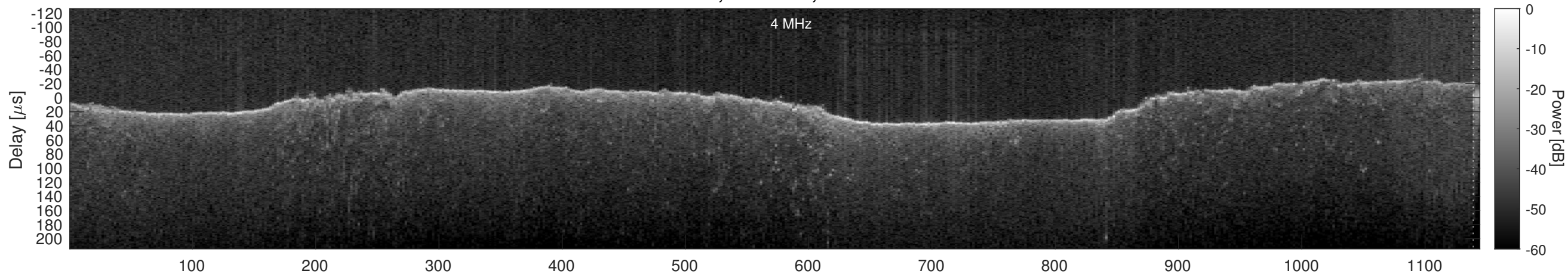
Orbit 15382, Window, Channel 1, Chapman
