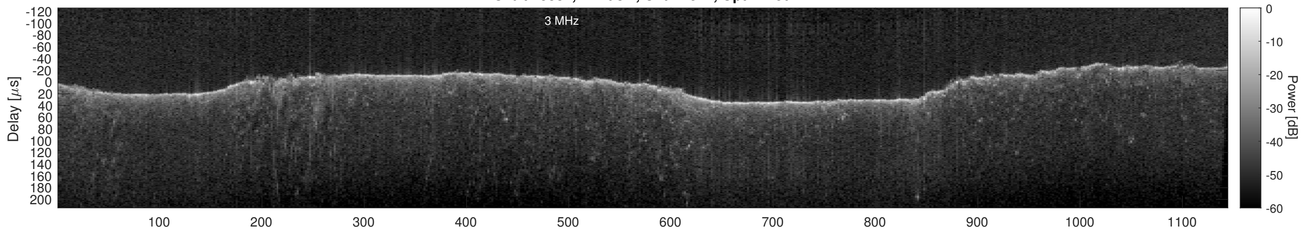
Orbit 15382, Cluttergram
