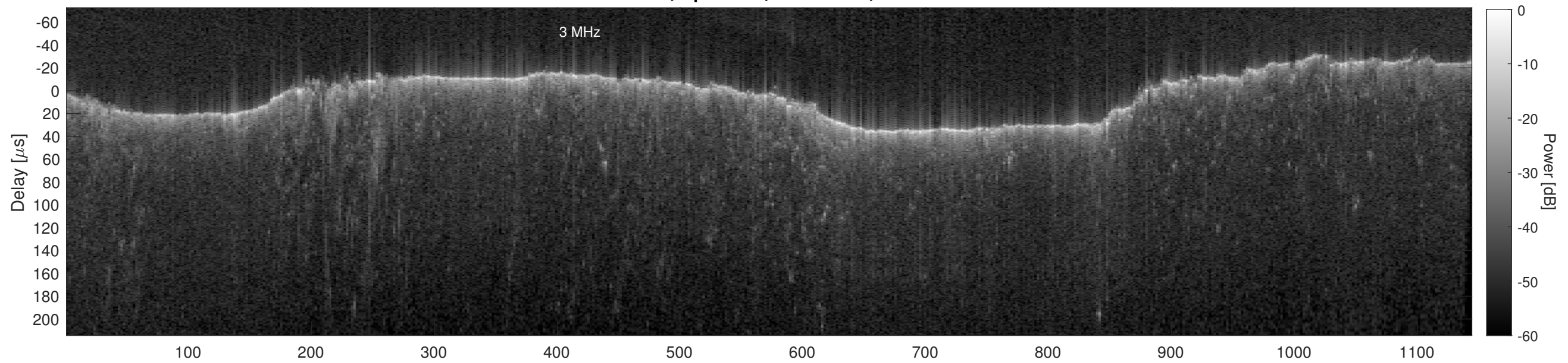
Orbit 15382, Cluttergram
