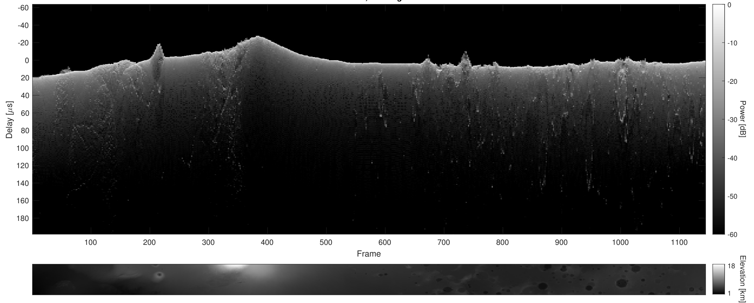
Orbit 15384, Cluttergram
