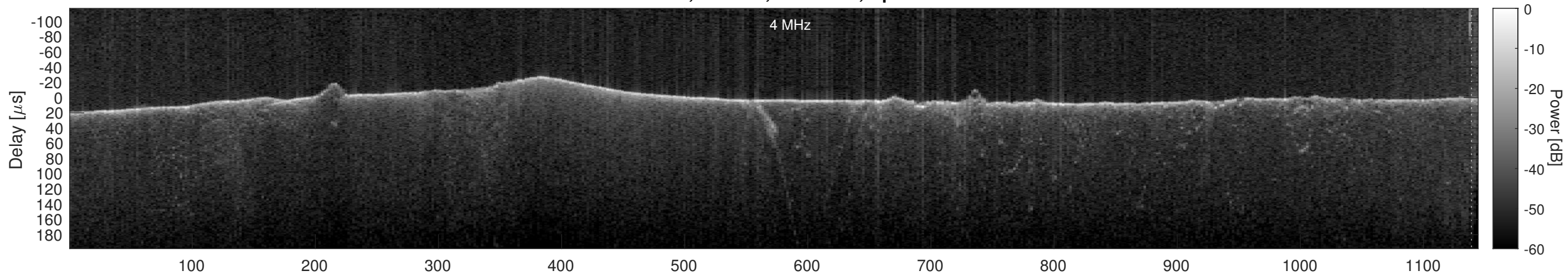
Orbit 15384, Cluttergram
