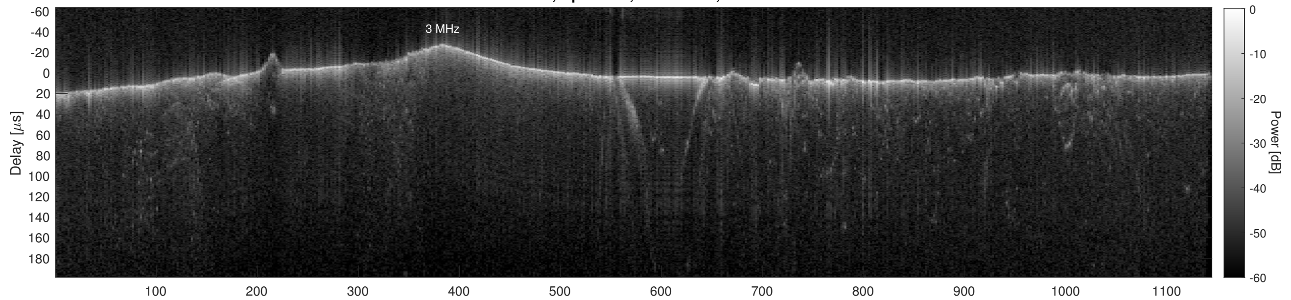
Orbit 15384, Cluttergram
