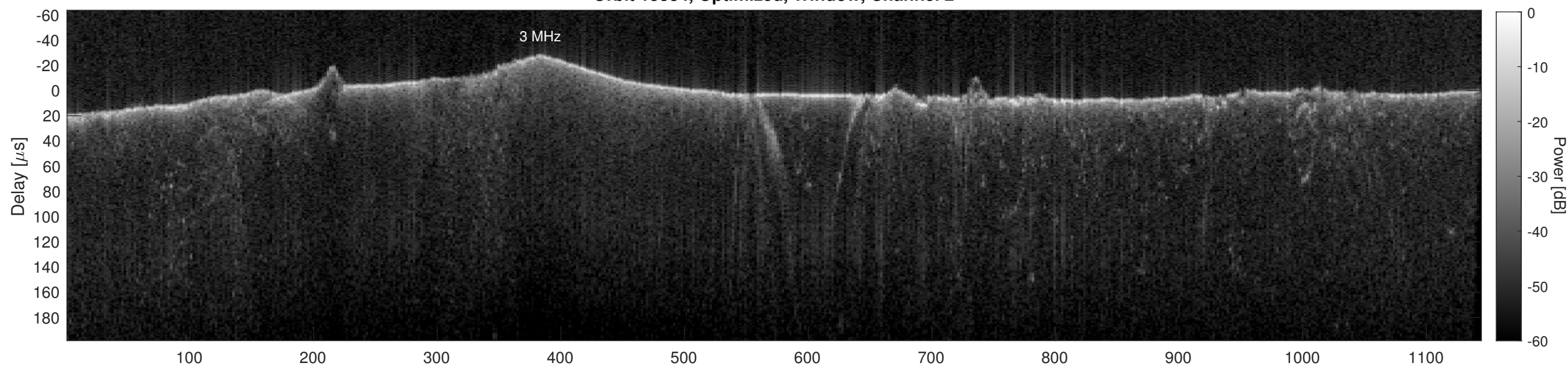
Orbit 15384, Cluttergram
