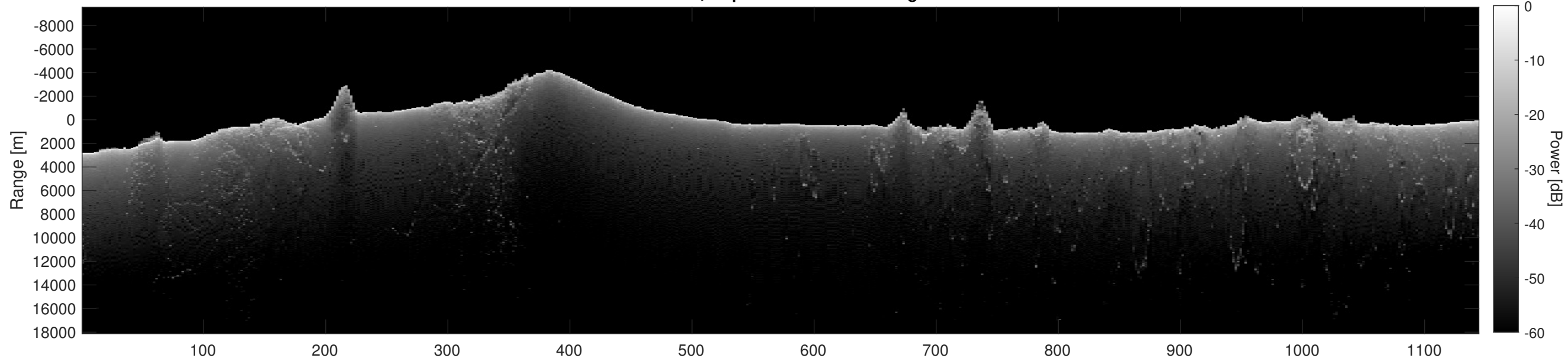
Orbit 15384, Depth-Corrected Cluttergram
