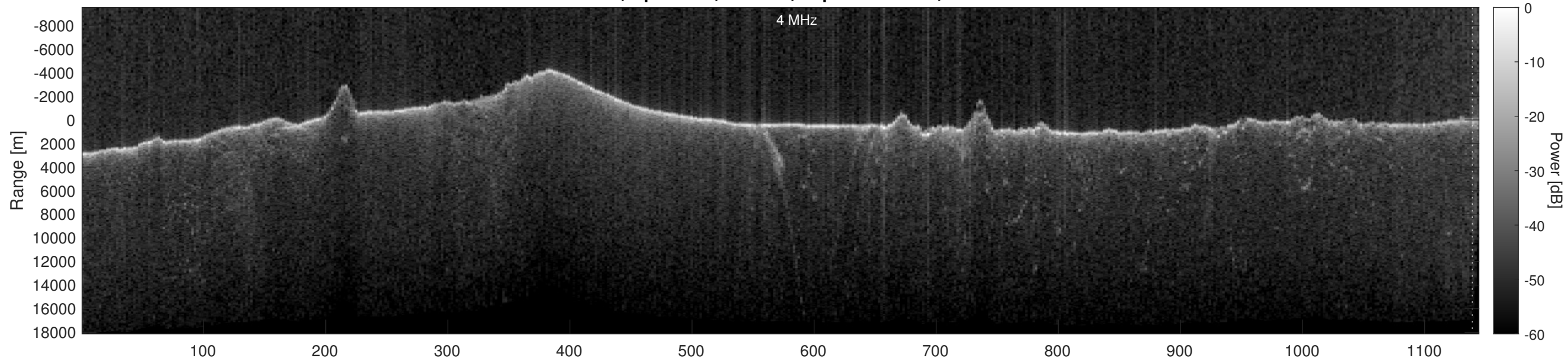
Orbit 15384, Optimized, Window, Depth-Corrected, Channel 2
