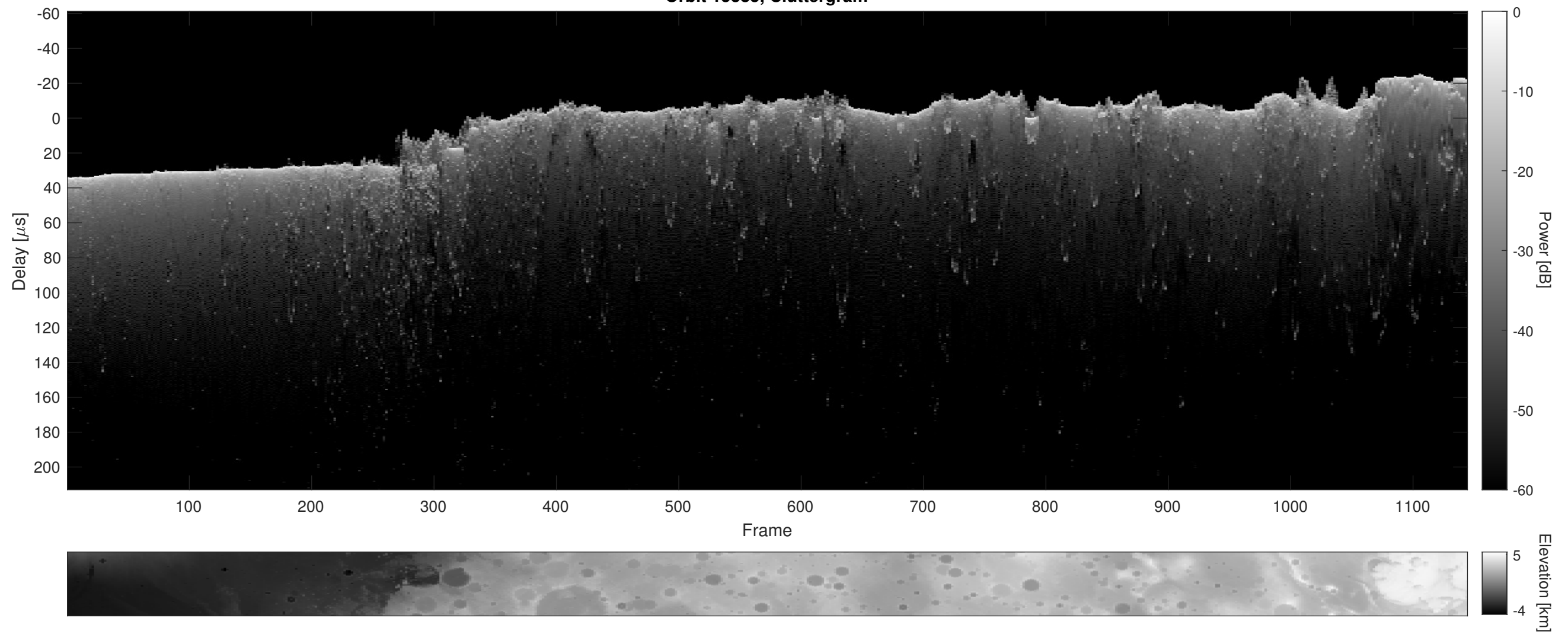
Orbit 15385, Cluttergram
