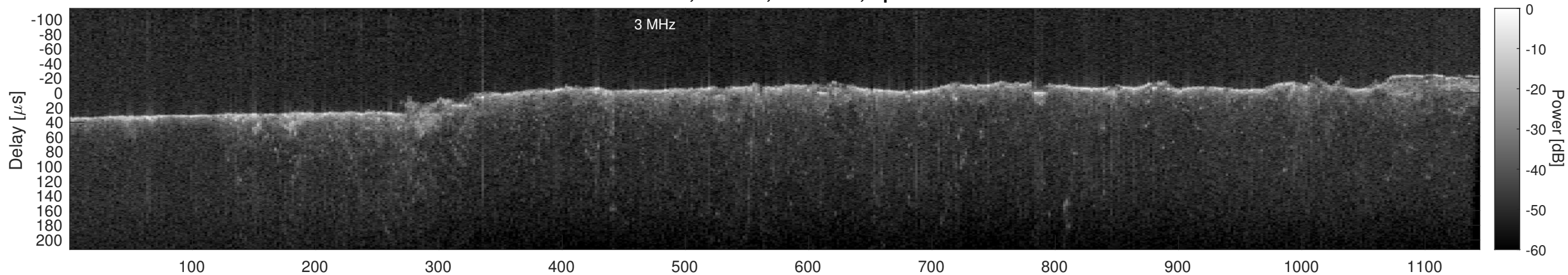
Orbit 15385, Cluttergram
