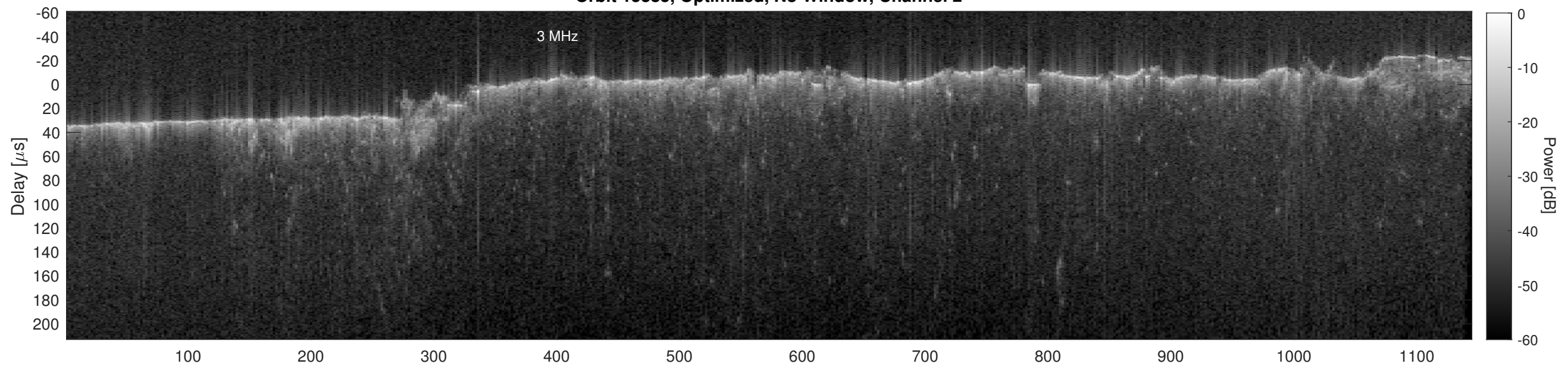
Orbit 15385, Cluttergram
